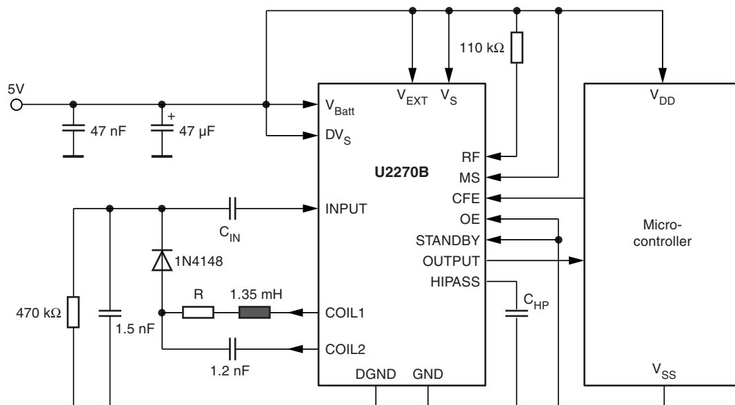
Figure 4-1. Application Circuit 1
